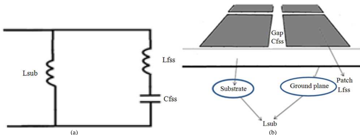
Fig.1. (a) Circuit representation for the HIS structure (b) Conventional Square-patch based HIS structure
